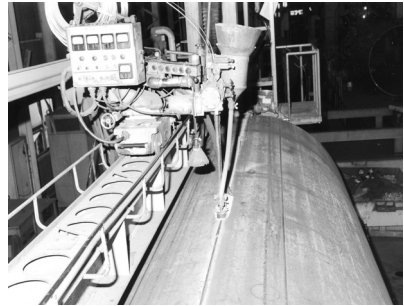
Outside Welding
