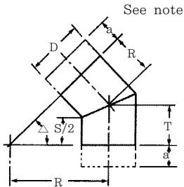
Two-Piece Elbow(0-45°)
