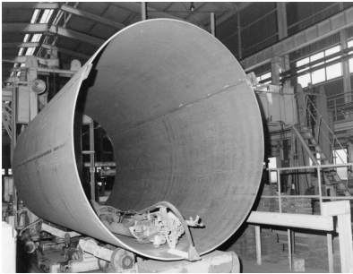
Inside Welding
