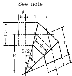
Three-Piece Elbow(30-90°)
