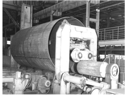
Roll Bending
